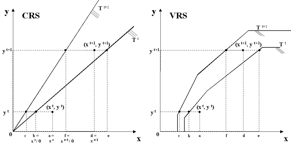
Figure 4: Input-oriented Malmquist approach for CRS and VRS
